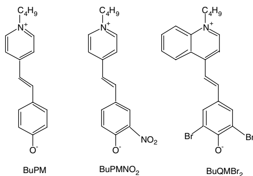
Figure 2. Solvatochromic probes BuPM, BuPMNO 2 and BuQMBR 2
