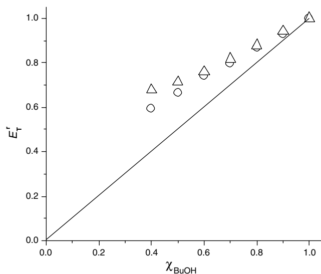
Figure 5. Dependence of E_T^r (BuQMBBr 2 ) on \chi_{\text{BuOH}} . The diagonal line represents the expected behavior if solvatochromism were ideal, i.e. if there were no preferential solvation of the probe: ( \Delta ) experimental results; ( \circ ) calculated contribution to E_T^r of dielectric enrichment (see Eqn (16) of the Calculations section)
