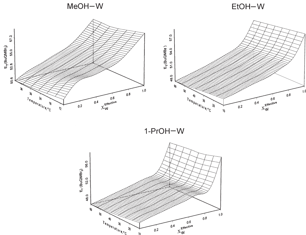
Figure 6. Solvent polarity/temperature/solvent composition contours for BuQMBr 2 in MeOH-W, EtOH-W and 1-PrOH-W, respectively
