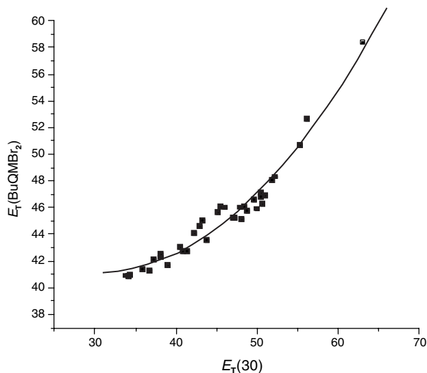
Figure 4. Correlation between the E_T(\text{BuQMBR}_2) and E_T(30) polarity scales, data at 25 °C
