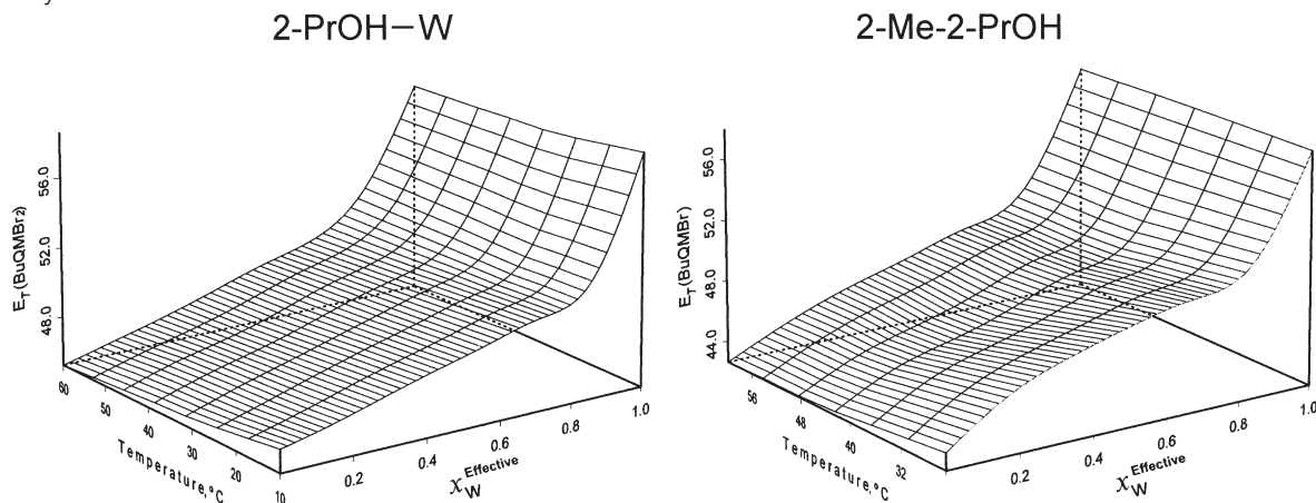
Figure 7. Solvent polarity/temperature/solvent composition contours for BuQMBr 2 in 2-PrOH-W and 2-Me-2-PrOH-W, respectively
