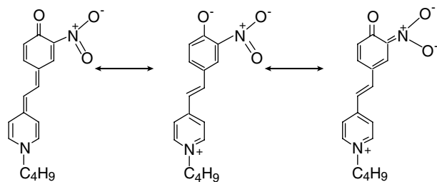
Figure 3. Resonance structures of BuPMNO 2
