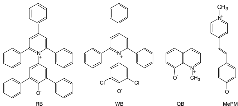
Figure 1. Structures of some previously employed solvatochromic probes; their pK_a values are 8.32, 4.78, 6.80 and 8.37, respectively
